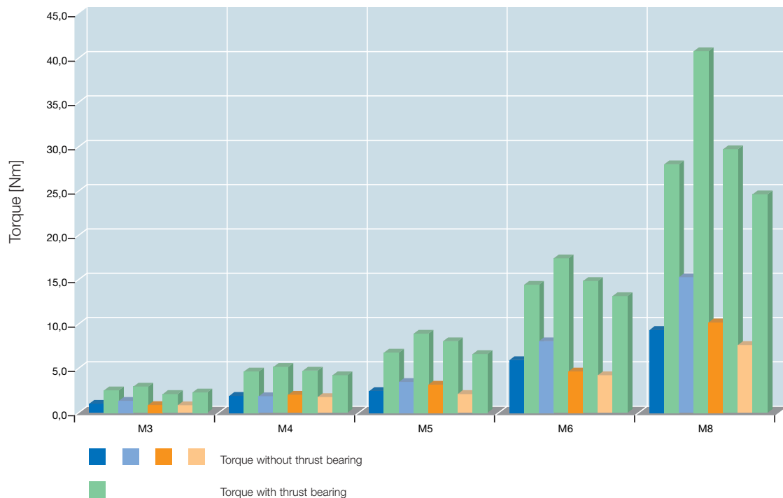
Torque values SONICSERT® M 3 to M 8
